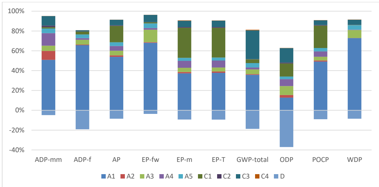
Figure 2: Tensor® TriAx® TX150L-GD - Impact of the individual modules on the environmental core indicator
