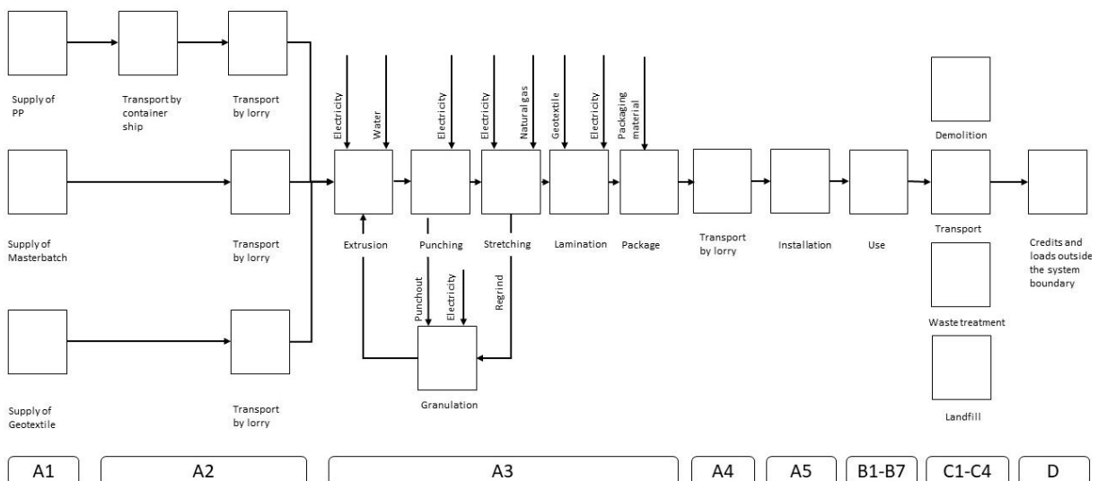
Figure 1: Process flow chart of the production of Tensor® TriAx® TX100-G series
